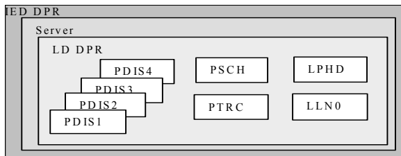
Figure 6. Distance protection relay model
