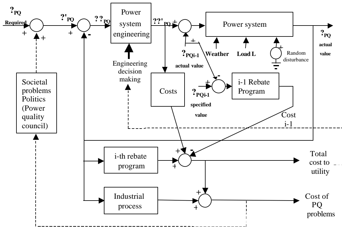
Figure (2) Conceptual diagram of power quality control system
