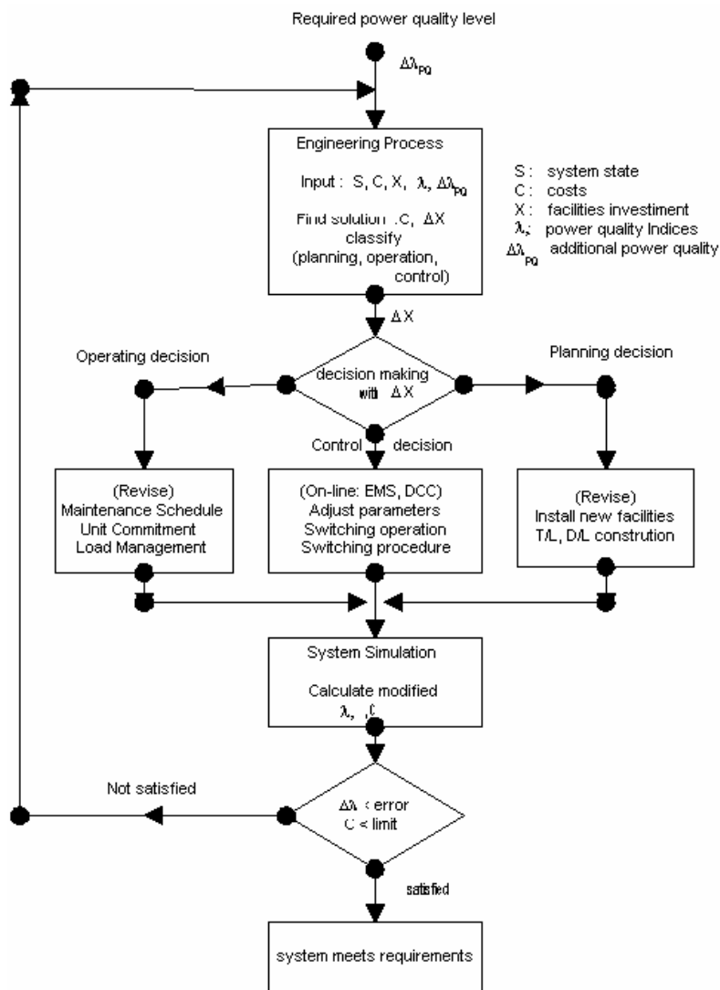
Figure (3) Engineering process for power quality
